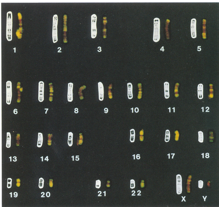
FIG. 3. (Left) A human metaphase spread hybridized with pooled fractions 7-9. (Right) The human haploid male karyotype constructed from the metaphase shown in Left. The right member of each chromosome pair in the reconstructed karyotype shows the observed hybridization pattern; the left member shows the R-banded karyotype. Reproduced from ref. 21 with permission (copyright Karger, Basel).
