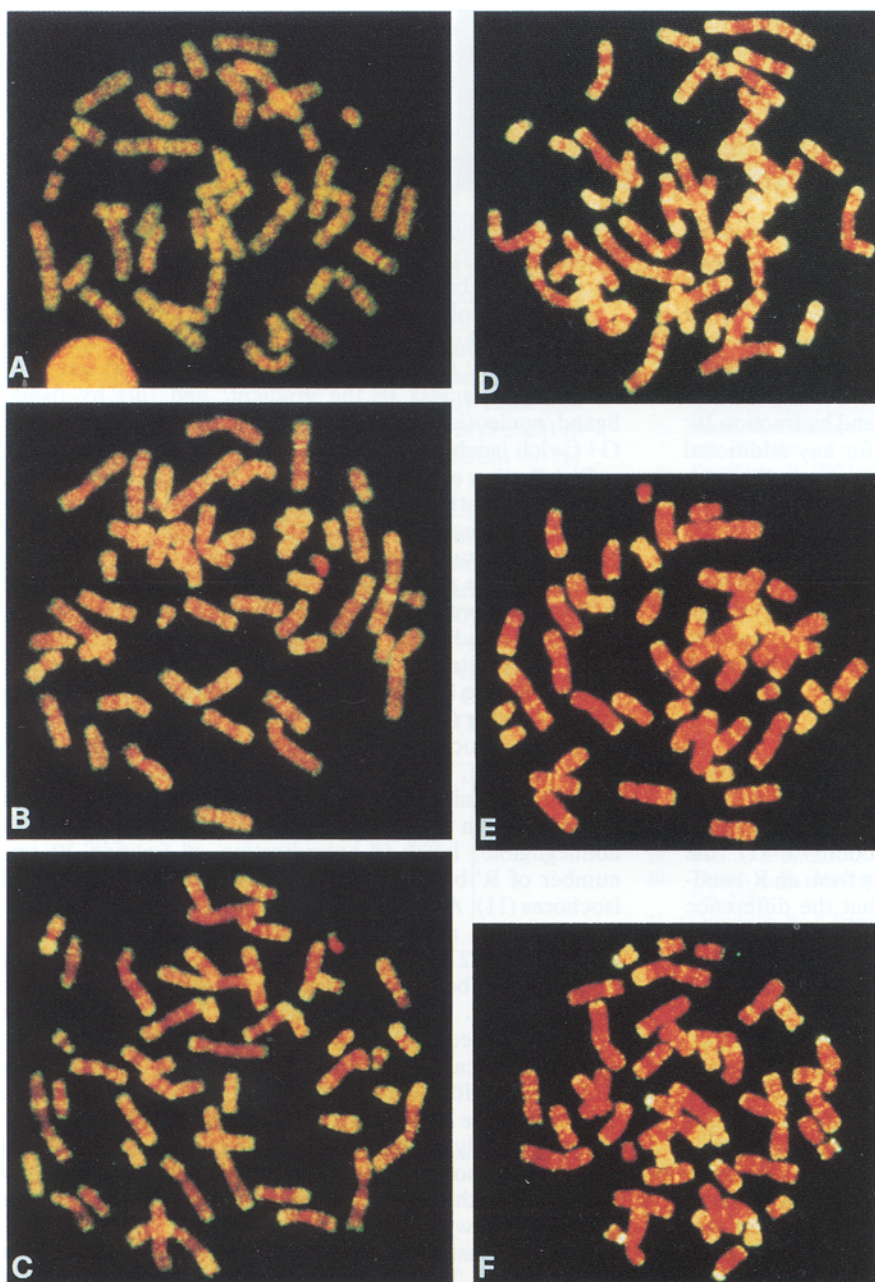
FIG. 2. In situ hybridization of aliquots of human DNA fractions on metaphase chromosomes. (A) Fractions 1–4, corresponding to the isochore families L1 + L2. (B–D) Fractions 5–7, corresponding to the isochore family H1. (E and F) Fractions 8 and 9, corresponding to isochore family H2. Detection of biotinylated probes was obtained with fluorescein isothiocyanate-conjugated avidin (yellow), and chromosomes were stained with propidium iodide (red).
