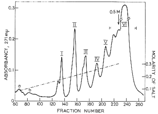
FIGURE 3: Chromatography of an acid DNase digest (A, see Tables I and II) of calf thymus DNA ( 170A_{271} units) on a DEAE-cellulose (chloride) column ( 1.8 \times 25.5 cm). DNA solution (650 ml) ( A_{260} 8.88) in SAB was digested with 20 \mu\text{l} of DNase HS 11 (undiluted, A_{280} 1.14) for 1 hr at room temperature; the sample was further digested with 10 \mu\text{l} of enzyme for 15 hr at room temperature. The digest was diluted with four volumes of water, adjusted to pH 8.0, and applied to the column. Collection of fractions was started immediately. Elution was carried out with a linear molarity gradient of NaCl: 0–0.3 M (2000 ml) in 7 M urea (pH 7.5). Fraction size, 8.5 ml; flow rate, 50 ml/hr. The continuous line indicates the absorption at 271 m\mu ; the broken line the molarity gradient.
