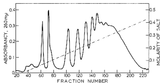
FIGURE 7: Chromatography of a dephosphorylated acid DNase digest D of calf thymus DNA (212 A_{271} units) on a DEAE-cellulose (chloride) column (1.3 × 43 cm). DNA solution (300 ml) ( A_{260} 8.13) in SAB was digested with 0.2 ml of concentrated acid DNase HS 17–18 ( A_{280} 4.4) for 5 hr at 25°. Inactivated digest (30 ml) was further digested in the same solvent with 1 ml of phosphomonoesterase I (activity/ml = 8) for 1 hr at 37°. After inactivation of the enzyme, 25 ml of the digest diluted 1:10 with distilled water and adjusted in pH 8.0 was applied to the column. Elution was carried out with linear molarity gradient of NaCl, 0–0.5 M (2500 ml), in 7 M urea (pH 7.5). Fraction size, 8.6 ml; flow rate, 50 ml/hr. Other indications as in Figure 3. See also Tables I and II.
