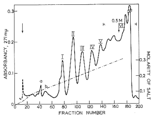
FIGURE 6: Chromatography of an acid DNase digest of H. influenzae DNA (111 A_{271} units) on a DEAE-cellulose (chloride) column (16 × 15 cm). DNA solution (50 ml) ( A_{260} 1.94) in SAB was digested with 0.5 ml of DNase HS 10 (1:100 dilution with 0.05% cytochrome c in SAB) for 1 hr at 37°; the sample was further digested with 0.5 ml for 3 hr at 37°. The digest was diluted with four volumes of water, adjusted to pH 8.0, and applied to the column. Elution was carried out with a linear molarity gradient of NaCl, 0–0.3 M (1000 ml), in 7 M urea (pH 7.5); 0.5 M NaCl was then used to elute the oligonucleotides left on the column. Fraction size 5.5 ml; flow rate, 68 ml/hr. Other indications as in Figure 3. See also Tables I and II.
