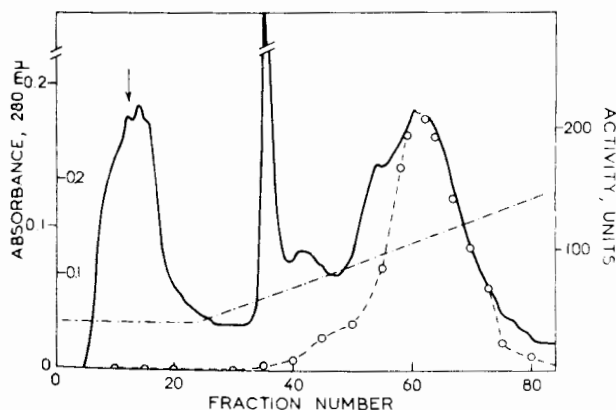
Fig. 4. Chromatography on CM-Sephadex C-50 of acid ribonuclease fractions from hydroxyapatite. 120 ml ( A_{280m\mu} = 0.67 ; A_{260m\mu} = 0.40 ) were loaded on a 2 cm \times 40 cm column of CM-Sephadex C-50 equilibrated with 0.05 M phosphate buffer (pH 6.0). Elution was carried out with a molarity gradient (0.05 to 0.4 M) of phosphate buffer. This was started at the fraction indicated by the arrow (left-hand inner scale). 10-ml fractions were collected. The continuous line indicates the absorption at 280 m \mu . Circles indicate the acid ribonuclease activity (right-hand scale). Fractions 58-72 were processed further.
