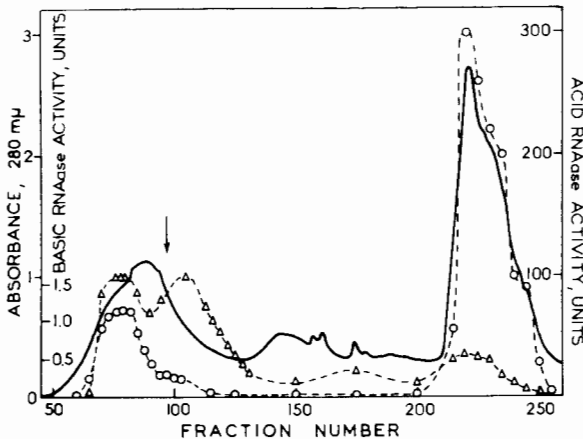
Fig. 1. Chromatography on DEAE-Sephadex A-50 of crude spleen nuclease II. 330 ml of preparation HS 9 ( A_{280m\mu} = 10.3 ; A_{260m\mu} = 6.9 ) were loaded on a 8 cm \times 80 cm column of DEAE-Sephadex A-50 equilibrated with 0.05 M phosphate buffer (pH 6.8). This buffer was also used to elute the first protein peak. 0.5 M phosphate buffer (pH 6.8) was applied at the fraction indicated by the arrow. 24-ml fractions were collected. The continuous line indicates the absorption at 280 m \mu . Circles indicate the acid ribonuclease activity (right-hand scale). Triangles indicate the basic ribonuclease activity (left-hand inner scale). Acid deoxyribonuclease, cytochrome c , acid phosphomonoesterase and phosphodiesterase were also assayed; the results are shown in Fig. 1 of refs. 5 and 7.
