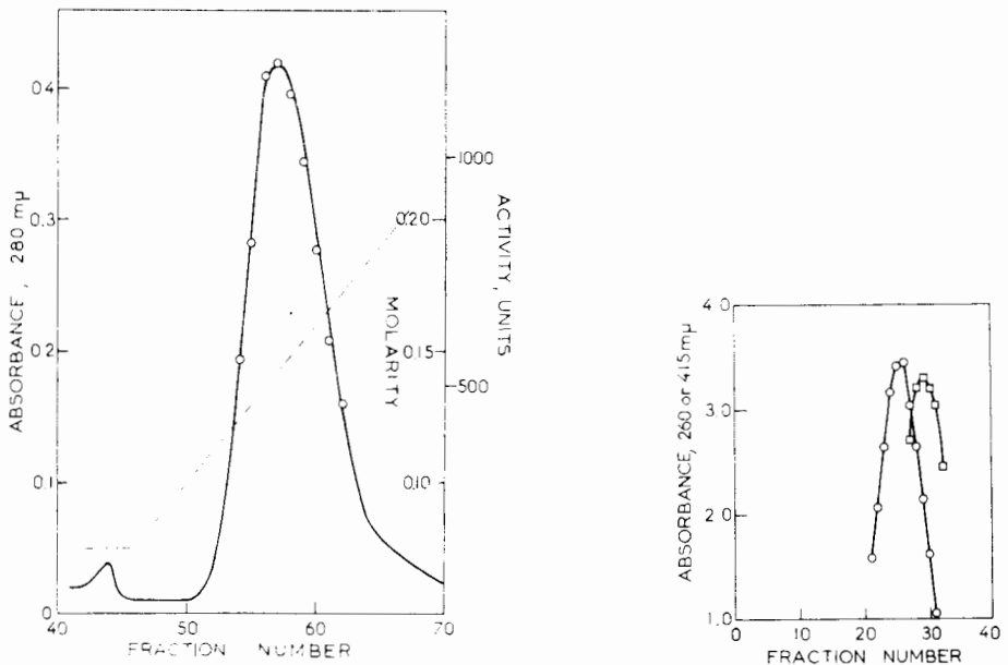
Fig. 5. Chromatography on hydroxyapatite of acid ribonuclease fractions from CM-Sephadex 183 ml ( A_{280m\mu} = 0.104 ; A_{260m\mu} = 0.064 ) are loaded on a 1 cm \times 13 cm hydroxyapatite column equilibrated with 0.05 M phosphate buffer (pH 6.8). A molarity gradient (0.1 to 0.3 M) of phosphate buffer was used to elute acid ribonuclease (right-hand inner scale). 4.6-ml fractions were collected. The continuous line indicates the absorption at 280 m\mu . Circles indicate the acid ribonuclease activity (right-hand scale). Fractions 53-60 were processed further.
