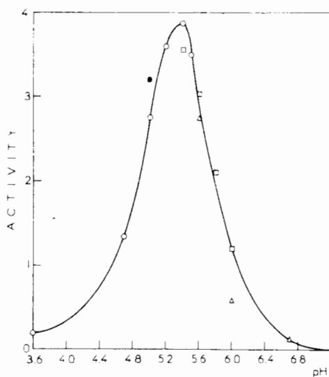
Fig. 9. Acid ribonuclease activity on soluble RNA; pH-activity curve at 37^\circ . The solvents were: 0.10 M NaCl-0.05 M acetate (circles), 0.05 M succinate (squares), 0.05 M phosphate (triangles), respectively. The activity measured when using 0.15 M acetate buffer (pH 5.0)-0.01 M EDTA is given for comparison (point).
